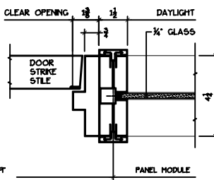
DOOR FRAME AT GLASS PANEL
