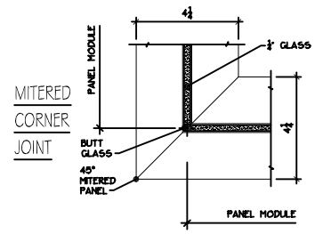
BUTT-END GLASS MITERED JOINT
